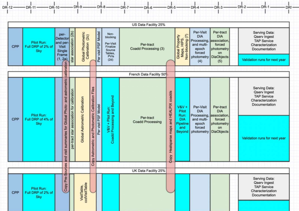
Figure 3: Timeline for a typical Data Release Processing Campaign 4
