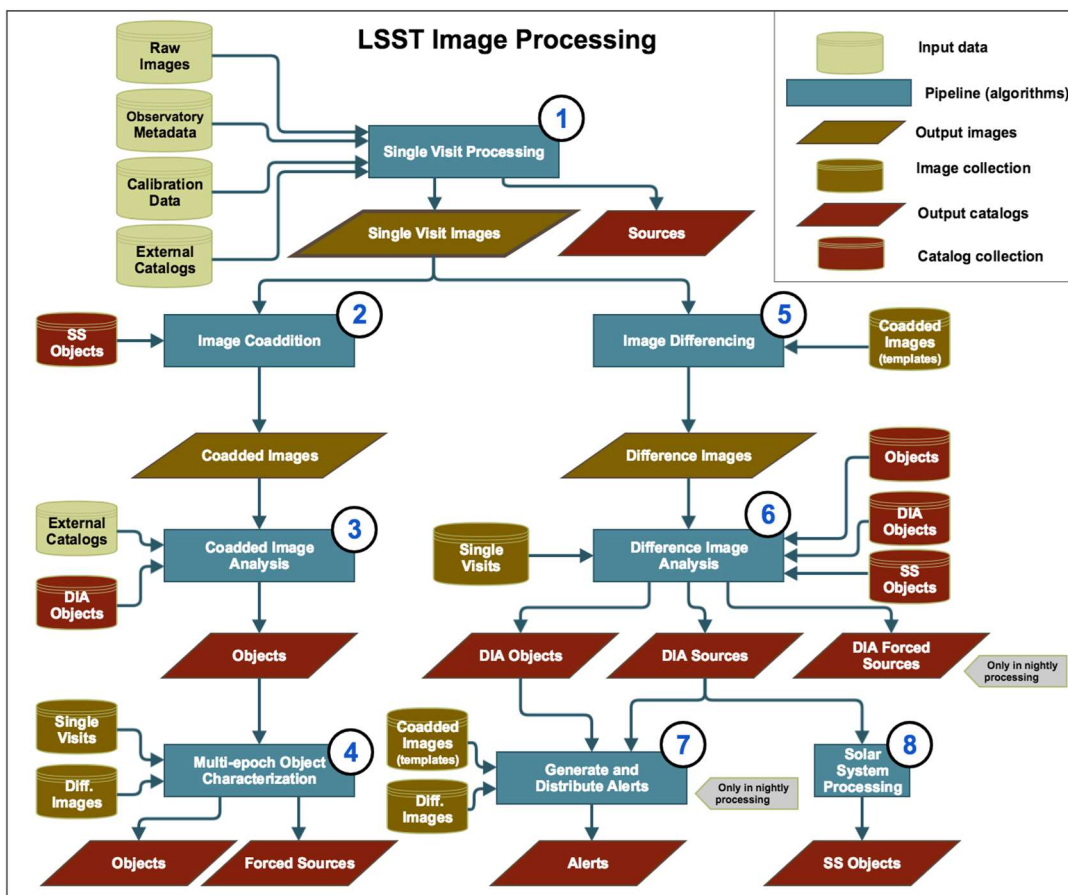
Figure 2: Stages of the Rubin Imaging Processing Pipeline
